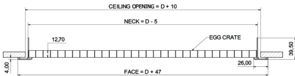
EGG CRATE GRILLE DIMENSIONS
